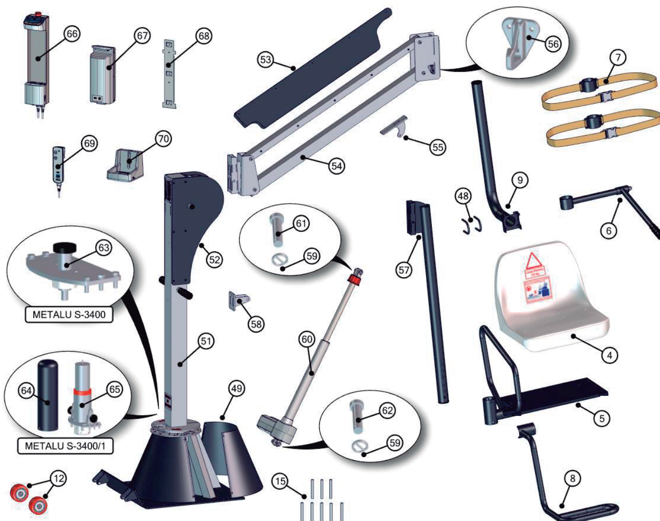
Exploded view and spare parts of the METALU S-3400 and S-3400/1 lift models.
